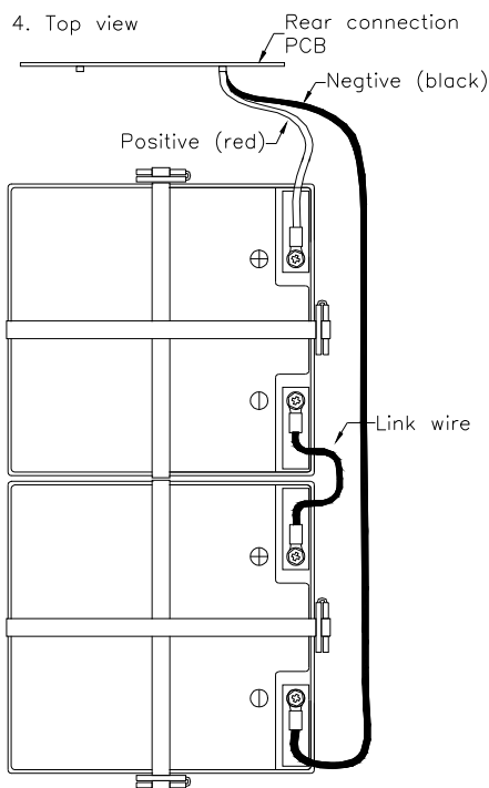
SBS241 Battery wiring layout
