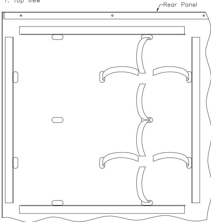
SBS241 Battery strap positions
