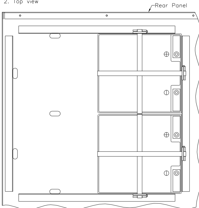
SBS241 Batteries strapped into position
